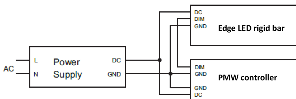
Figure 2: with controller
